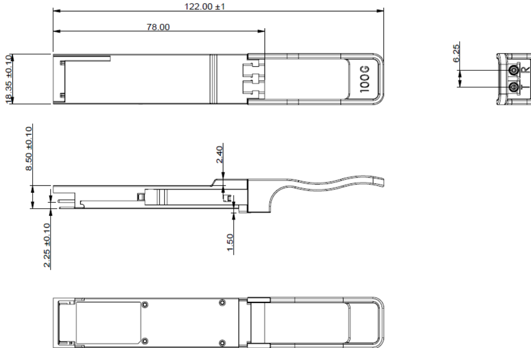
Figure 4. Mechanical Outline
