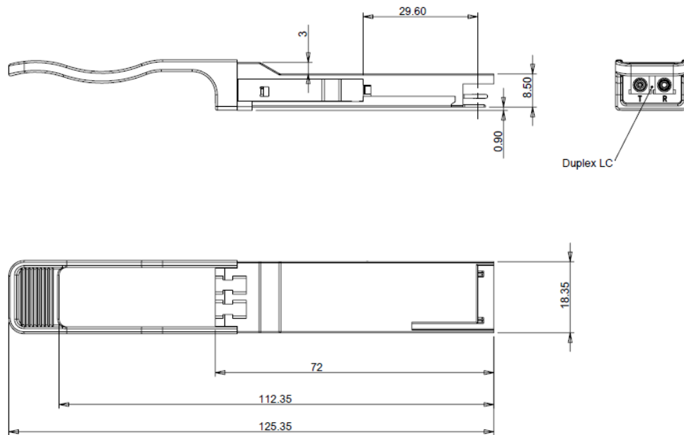
Figure 4. Mechanical Outline
