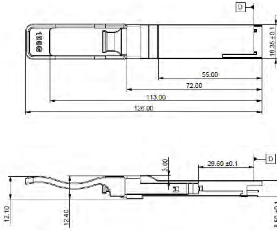
Figure 5. Mechanical Outline
