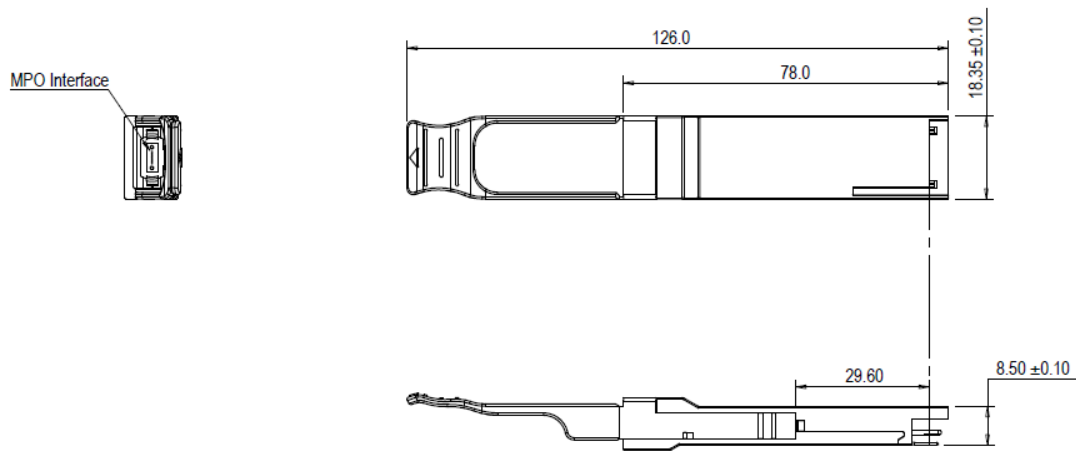
Figure 4. Mechanical Outline
